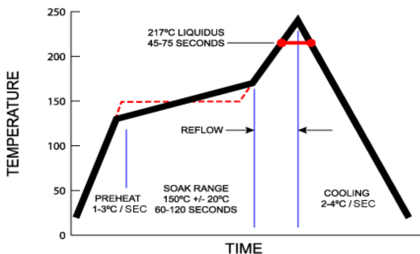
TYPICAL PROFILE FOR CONVENTIONAL LEAD FREE SOLDER
